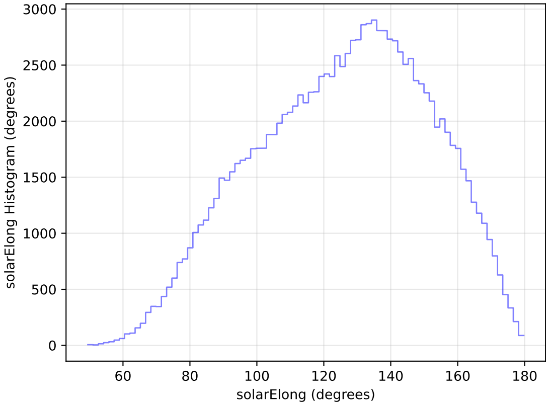
too_elab_heavy_r32_d2_gz_v3.4_10yrs WFD u band: solarElong Histogram
