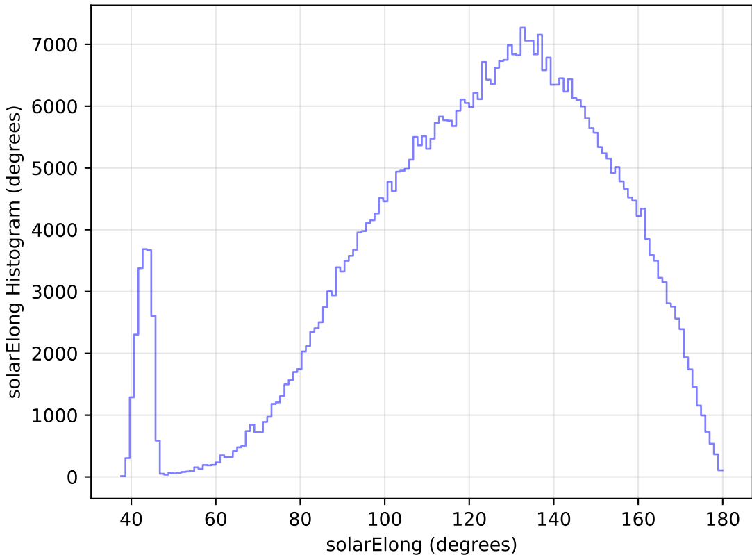
too_elab_heavy_r32_d2_gz_v3.4_10yrs WFD r band: solarElong Histogram
