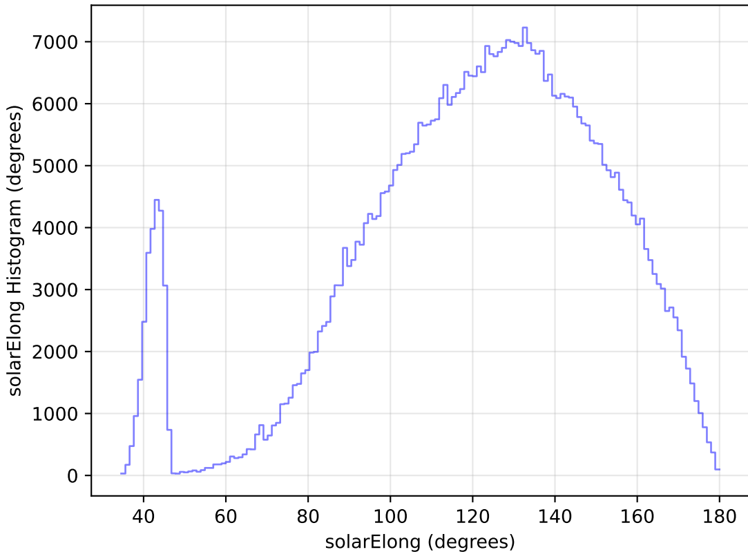
too_elab_heavy_r32_d2_gz_v3.4_10yrs WFD i band: solarElong Histogram
