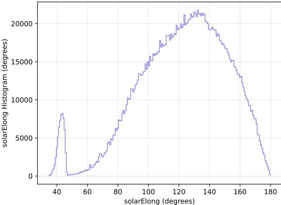
too_elab_heavy_r32_d2_gz_v3.4_10yrs WFD all bands: solarElong Histogram
