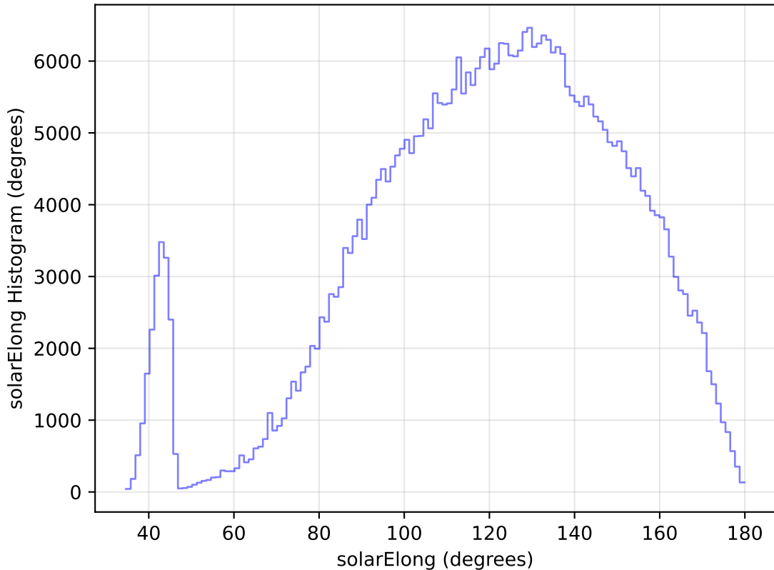
too_elab_heavy_r32_d2_gz_v3.4_10yrs All sky z band: solarElong Histogram
