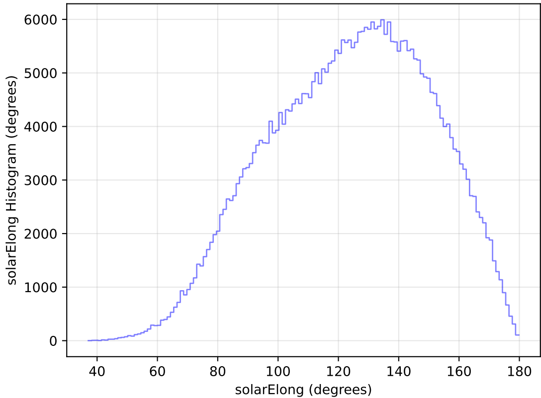
too_elab_heavy_r32_d2_gz_v3.4_10yrs All sky y band: solarElong Histogram
