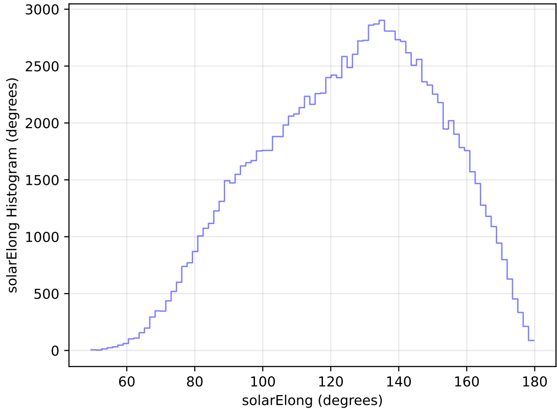
too_elab_heavy_r32_d2_gz_v3.4_10yrs All sky u band: solarElong Histogram
