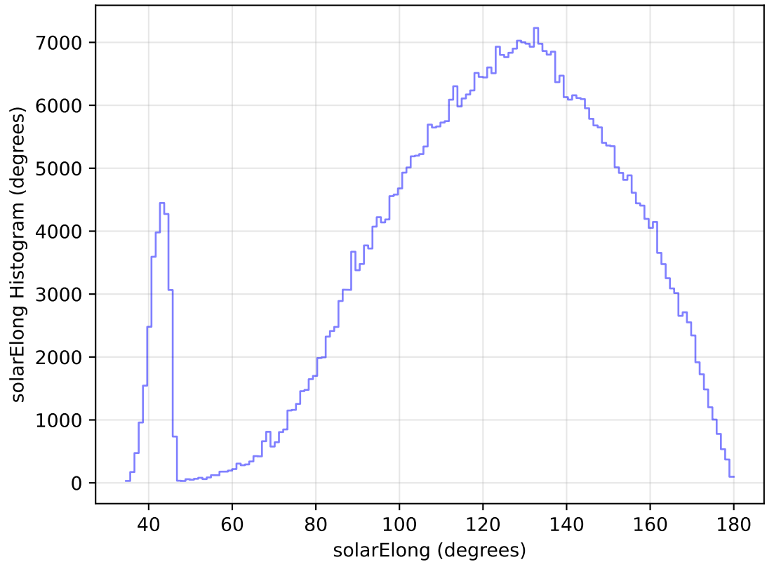
too_elab_heavy_r32_d2_gz_v3.4_10yrs All sky i band: solarElong Histogram
