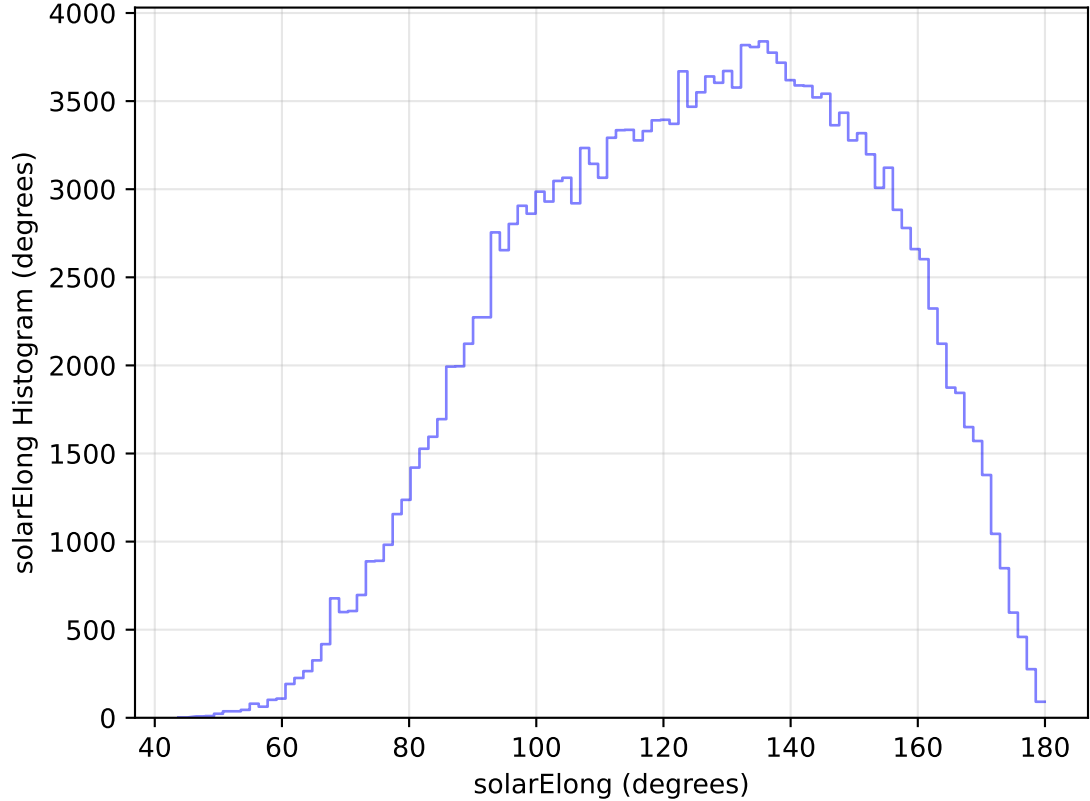
too_elab_heavy_r32_d2_gz_v3.4_10yrs All sky g band: solarElong Histogram
