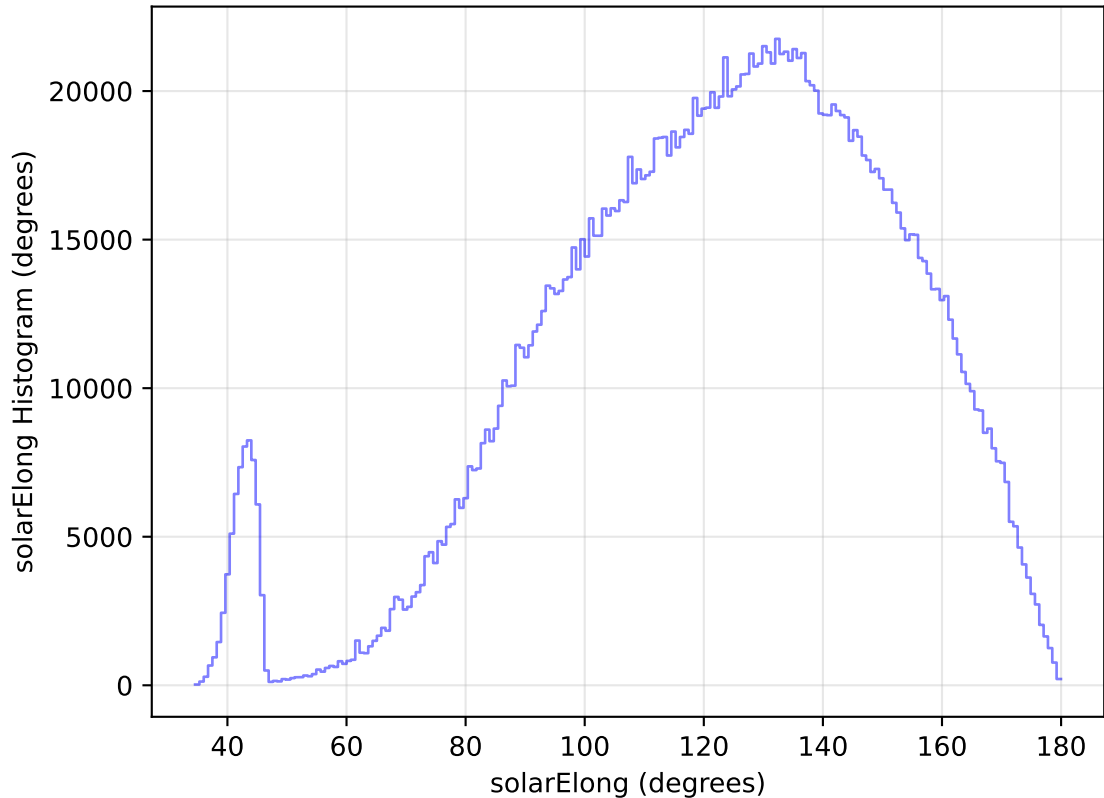
too_elab_heavy_r32_d2_gz_v3.4_10yrs All sky all bands: solarElong Histogram
