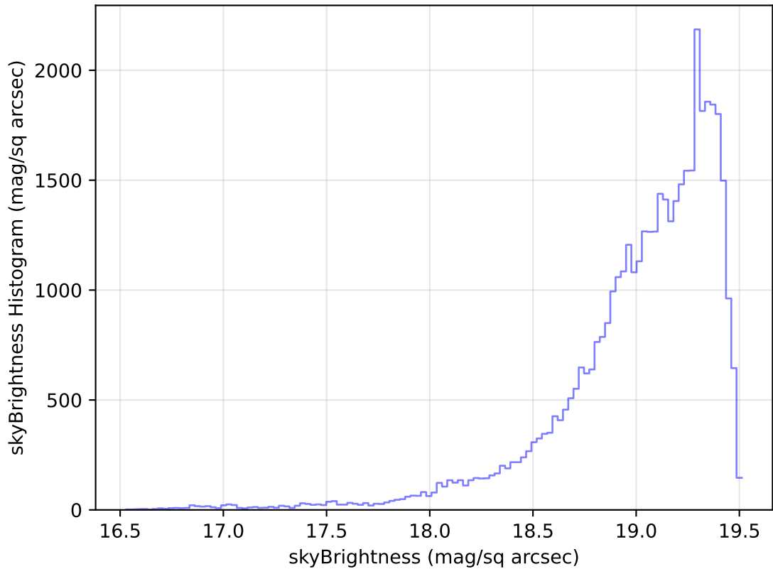
too_elab_heavy_r32_d2_gz_v3.4_10yrs Yr 1 z band: skyBrightness Histogram
