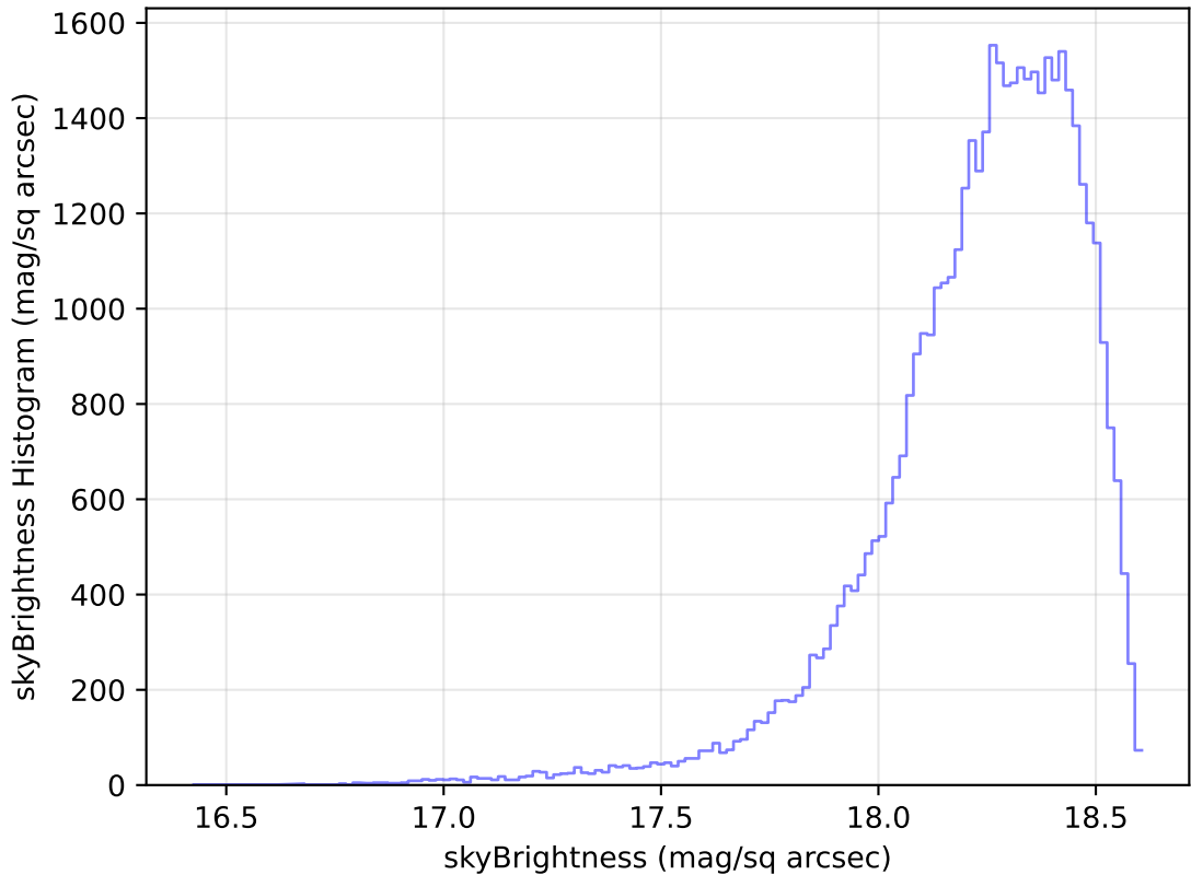
too_elab_heavy_r32_d2_gz_v3.4_10yrs Yr 1 y band: skyBrightness Histogram
