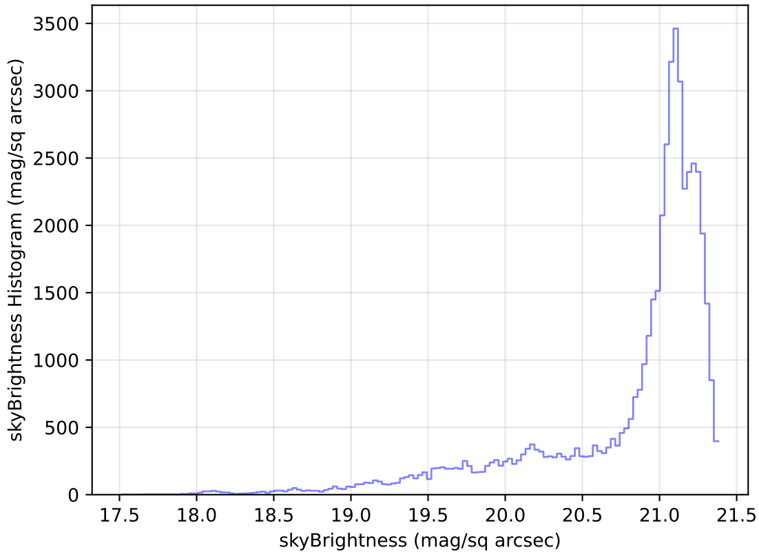
too_elab_heavy_r32_d2_gz_v3.4_10yrs Yr 1 r band: skyBrightness Histogram
