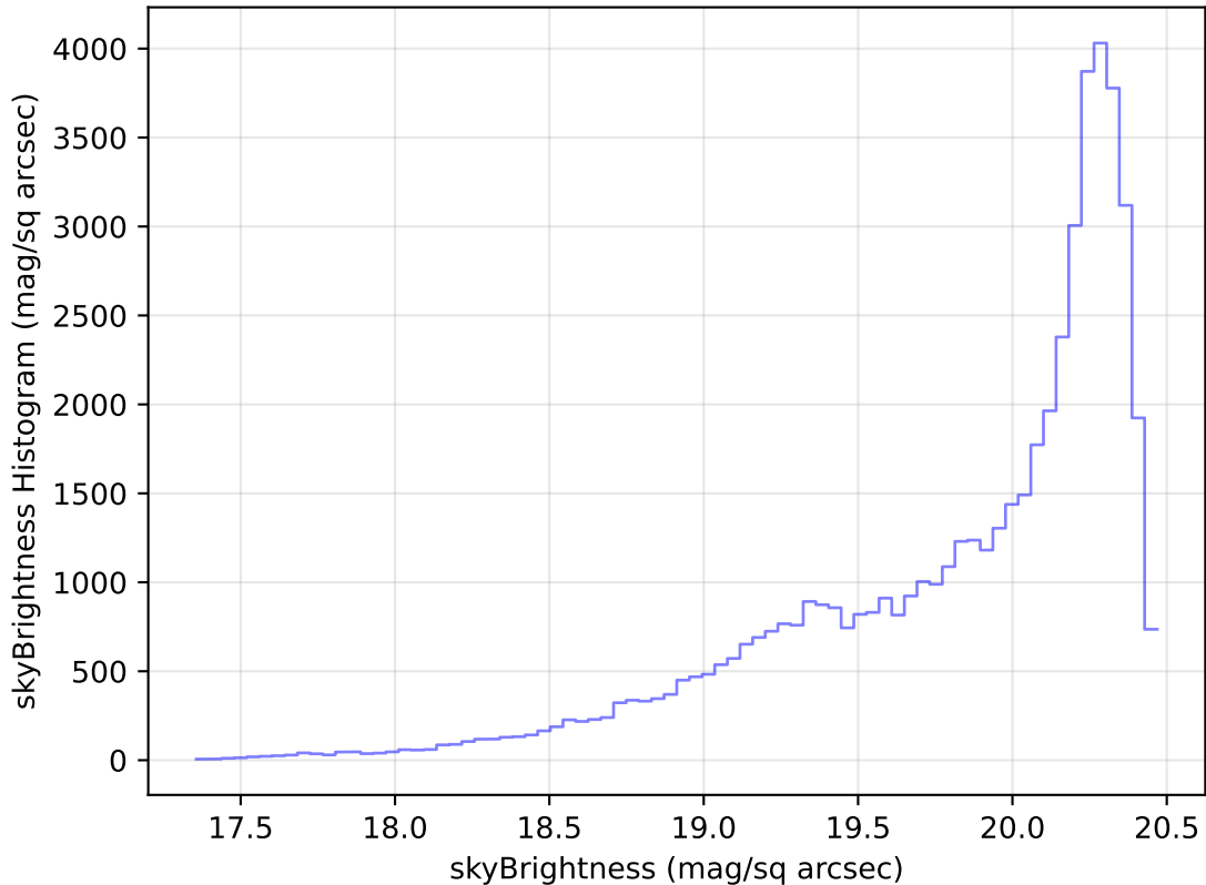
too_elab_heavy_r32_d2_gz_v3.4_10yrs Yr 1 i band: skyBrightness Histogram
