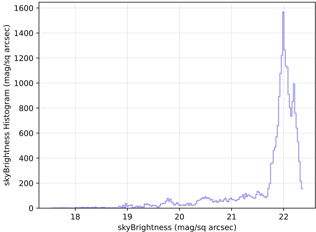
too_elab_heavy_r32_d2_gz_v3.4_10yrs Yr 1 g band: skyBrightness Histogram
