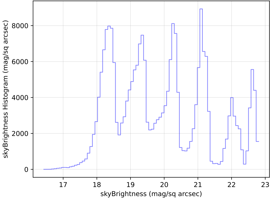
too_elab_heavy_r32_d2_gz_v3.4_10yrs Yr 1 all bands: skyBrightness Histogram
