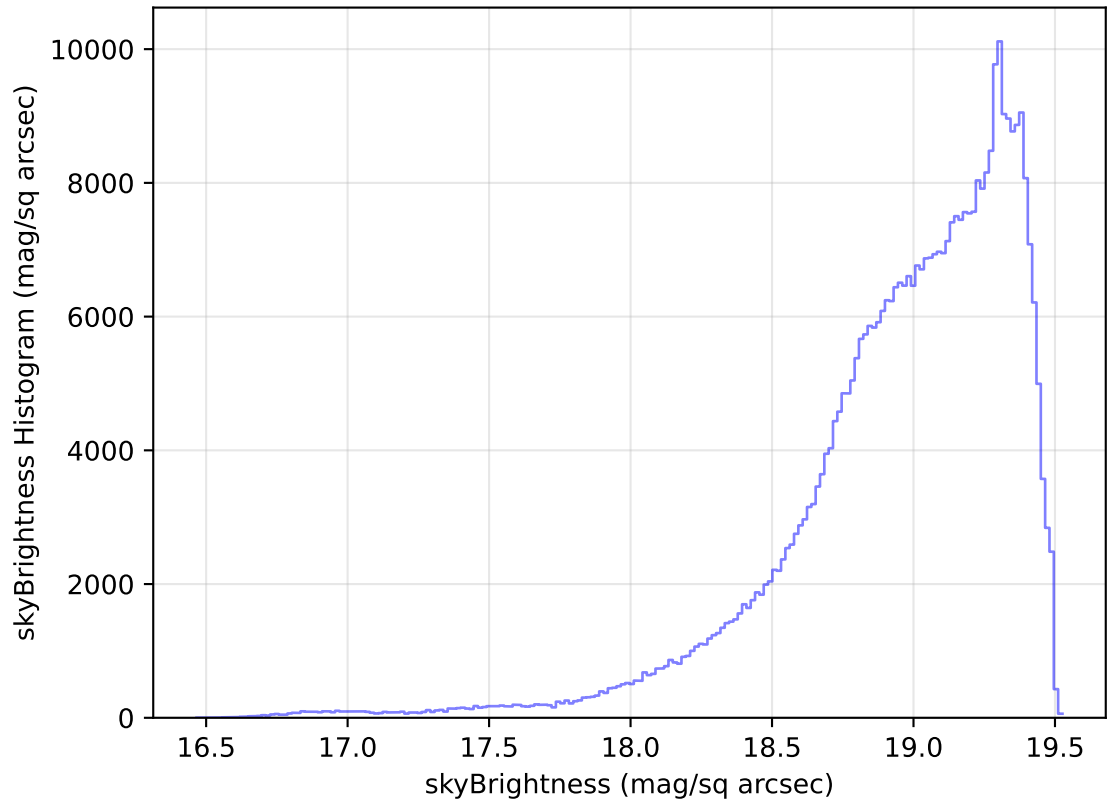
too_elab_heavy_r32_d2_gz_v3.4_10yrs WFD z band: skyBrightness Histogram
