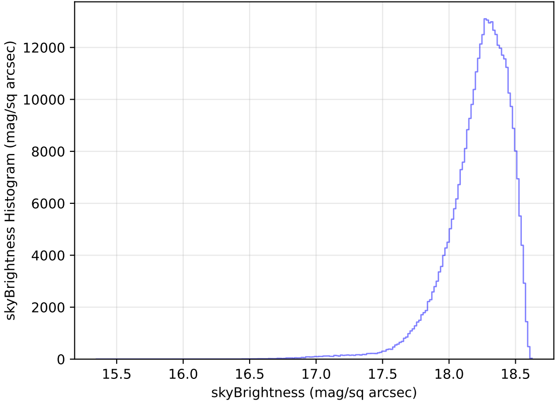
too_elab_heavy_r32_d2_gz_v3.4_10yrs WFD y band: skyBrightness Histogram
