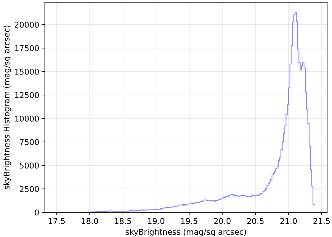
too_elab_heavy_r32_d2_gz_v3.4_10yrs WFD r band: skyBrightness Histogram
