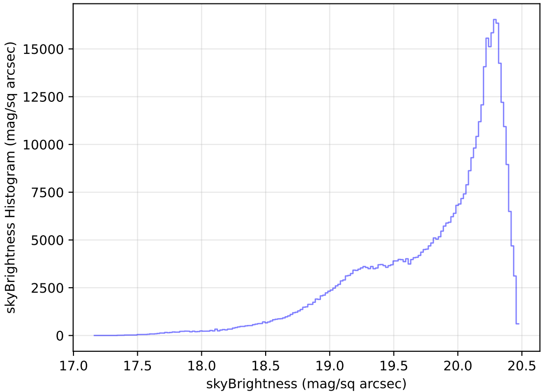
too_elab_heavy_r32_d2_gz_v3.4_10yrs WFD i band: skyBrightness Histogram
