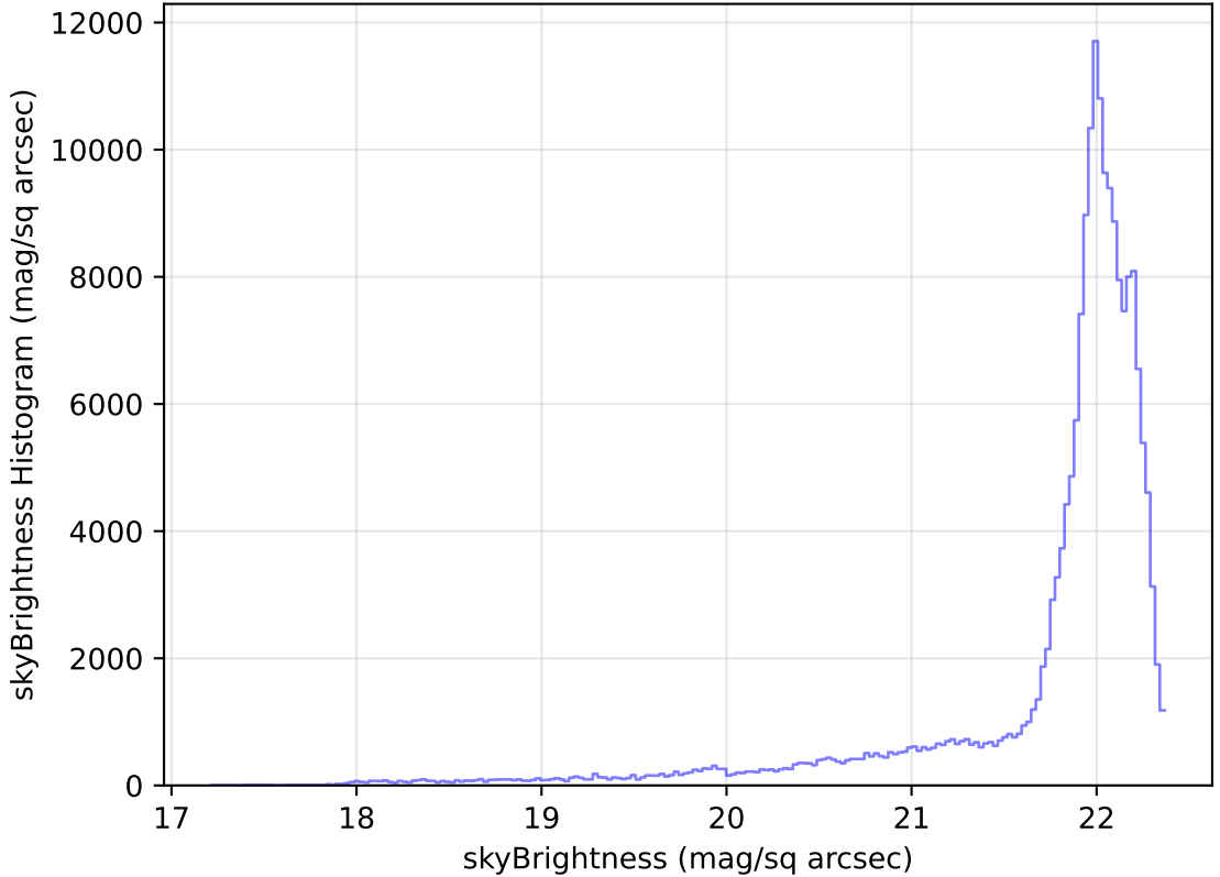
too_elab_heavy_r32_d2_gz_v3.4_10yrs WFD g band: skyBrightness Histogram
