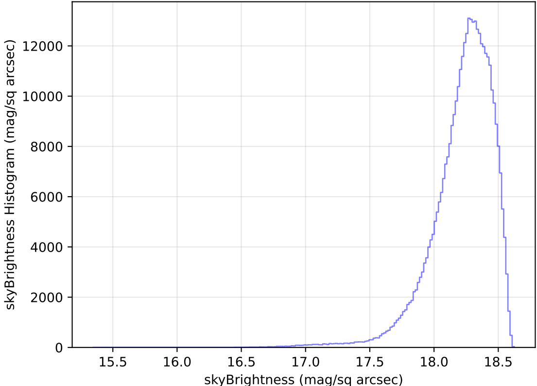
too_elab_heavy_r32_d2_gz_v3.4_10yrs All sky y band: skyBrightness Histogram
