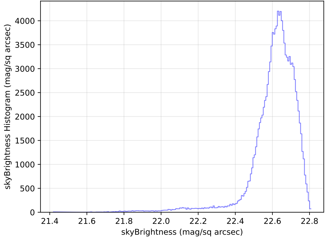
too_elab_heavy_r32_d2_gz_v3.4_10yrs All sky u band: skyBrightness Histogram
