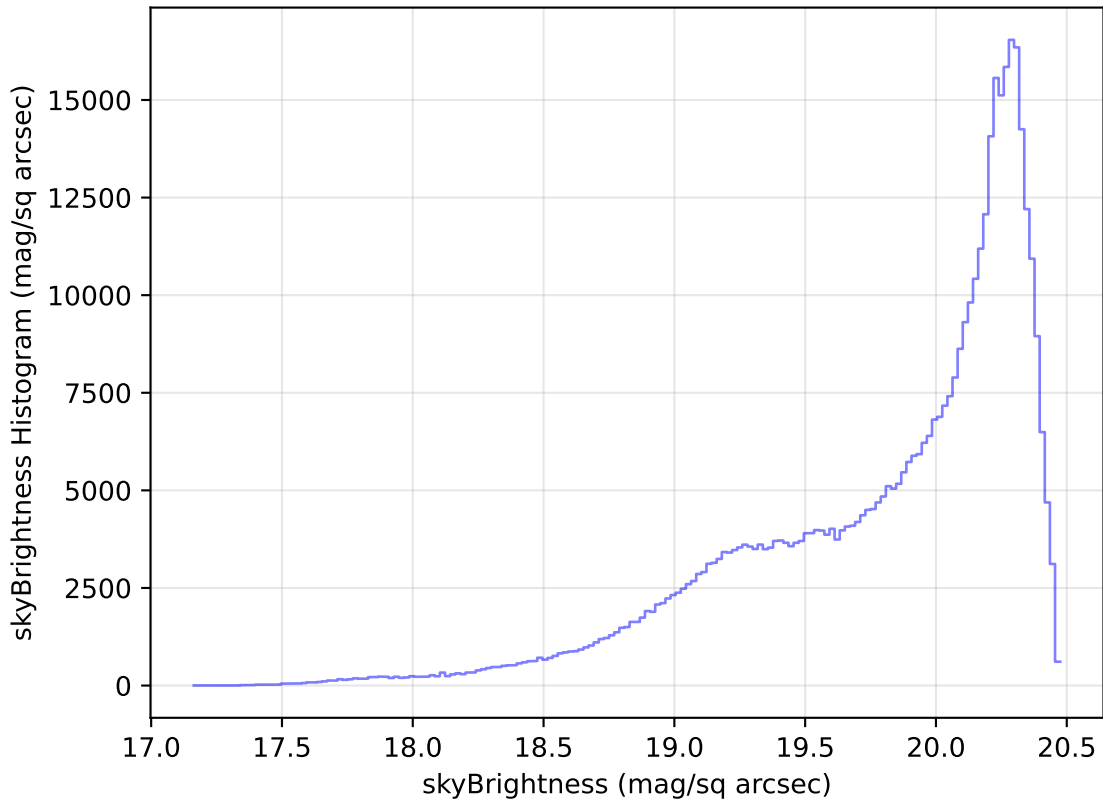
too_elab_heavy_r32_d2_gz_v3.4_10yrs All sky i band: skyBrightness Histogram
