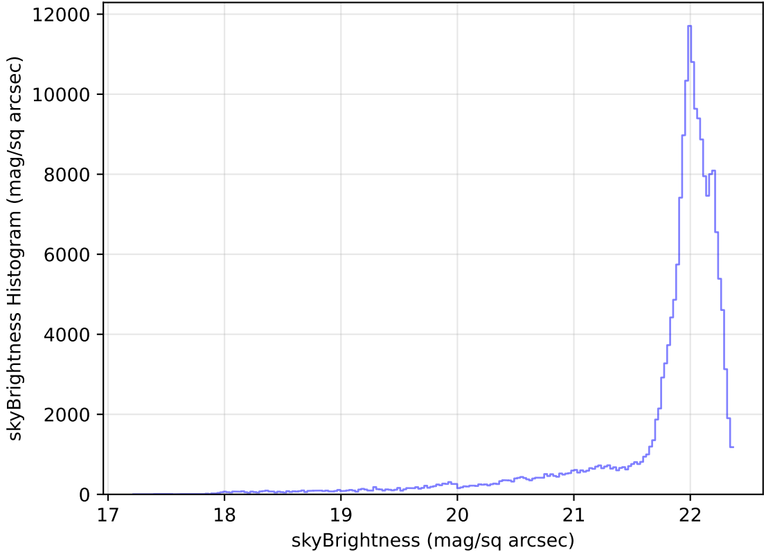
too_elab_heavy_r32_d2_gz_v3.4_10yrs All sky g band: skyBrightness Histogram
