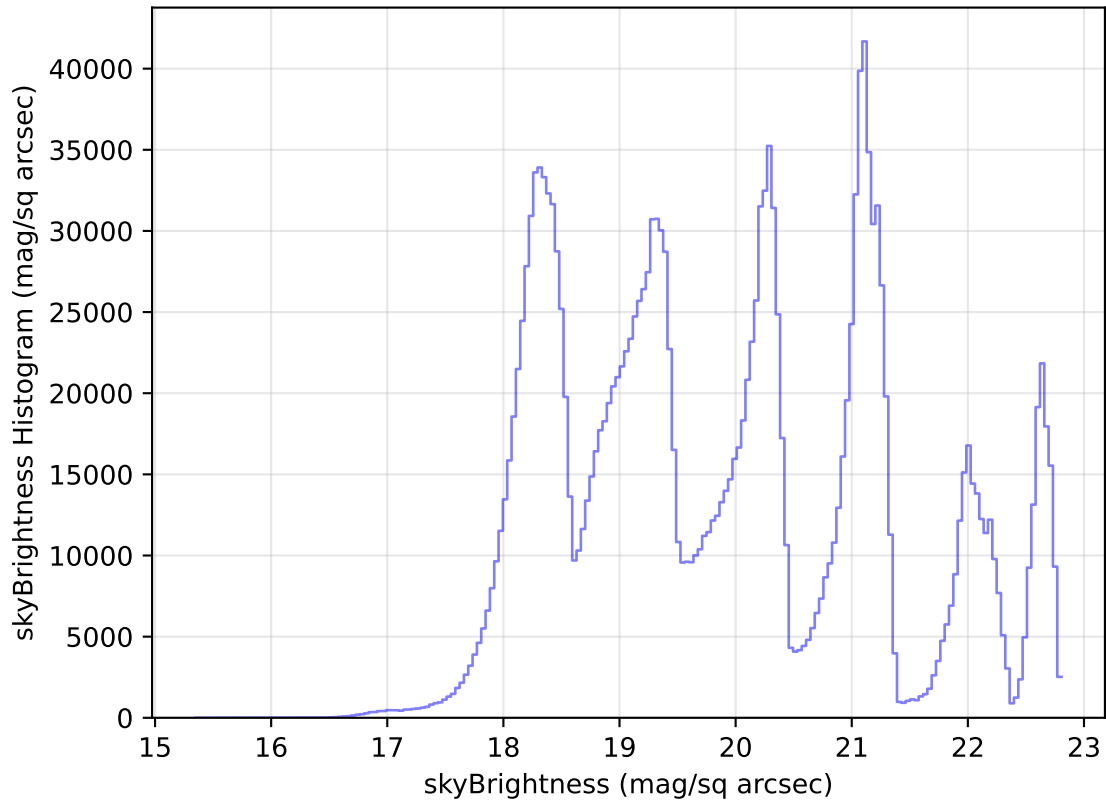
too_elab_heavy_r32_d2_gz_v3.4_10yrs All sky all bands: skyBrightness Histogram
