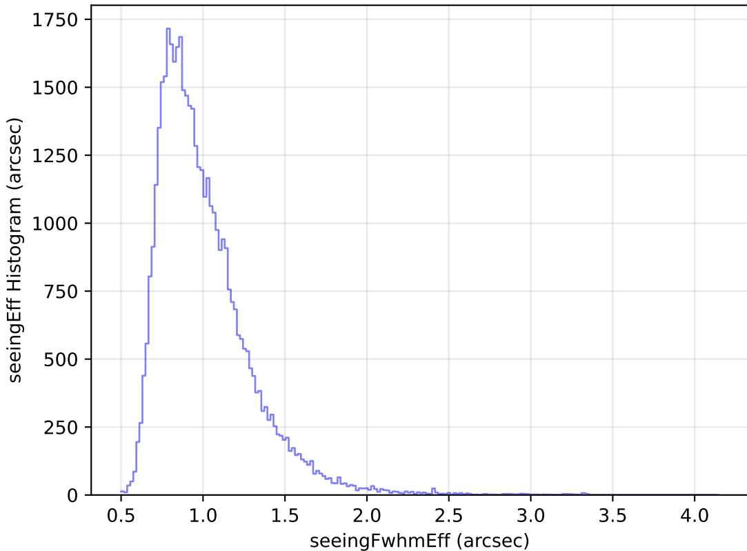
too_elab_heavy_r32_d2_gz_v3.4_10yrs Yr 1 z band: seeingEff Histogram
