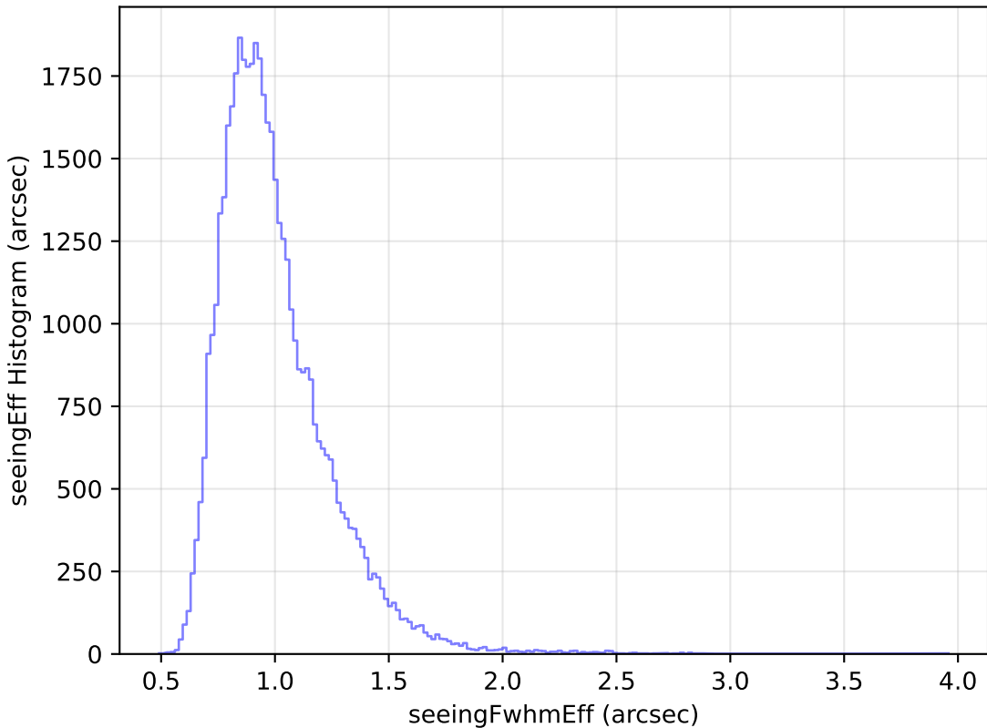
too_elab_heavy_r32_d2_gz_v3.4_10yrs Yr 1 y band: seeingEff Histogram
