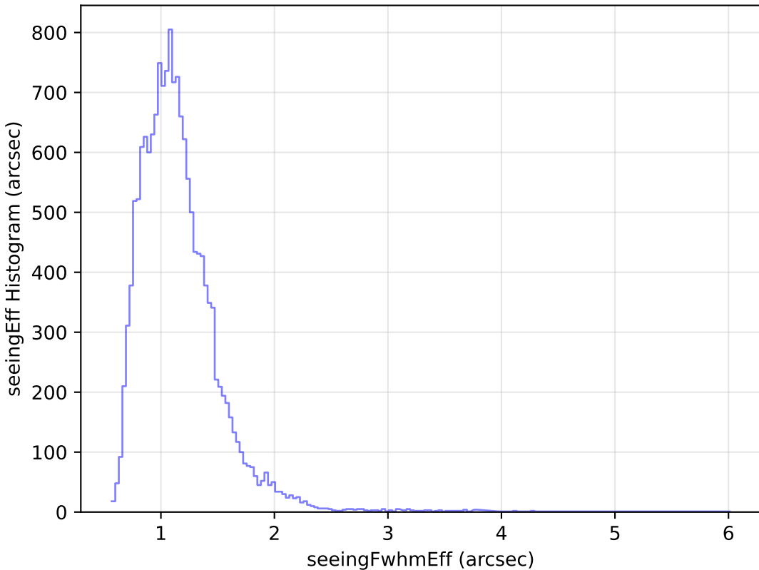
too_elab_heavy_r32_d2_gz_v3.4_10yrs Yr 1 u band: seeingEff Histogram
