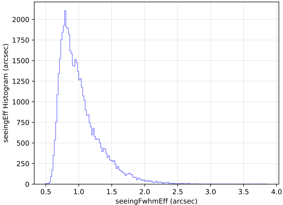
too_elab_heavy_r32_d2_gz_v3.4_10yrs Yr 1 r band: seeingEff Histogram
