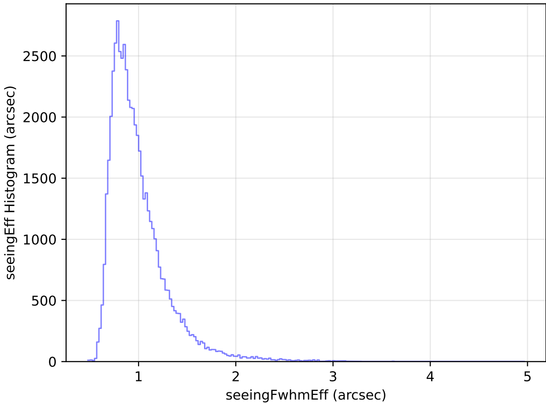
too_elab_heavy_r32_d2_gz_v3.4_10yrs Yr 1 i band: seeingEff Histogram
