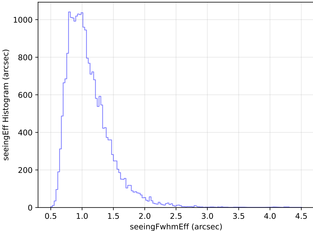
too_elab_heavy_r32_d2_gz_v3.4_10yrs Yr 1 g band: seeingEff Histogram
