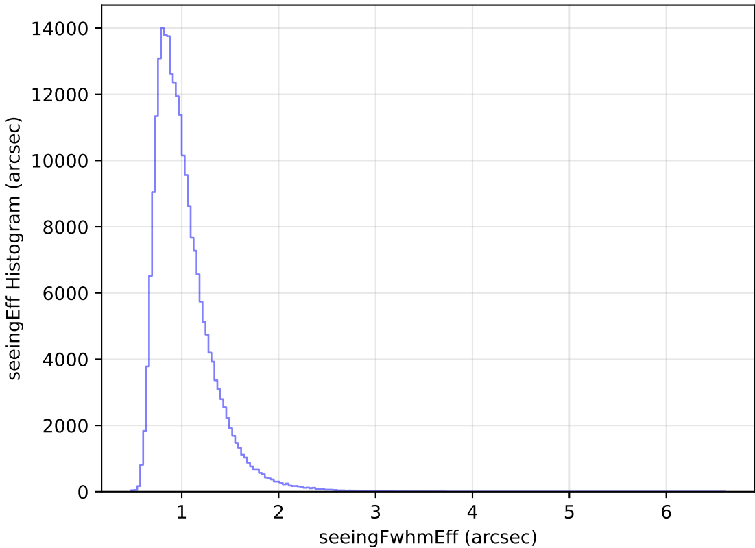
too_elab_heavy_r32_d2_gz_v3.4_10yrs Yr 1 all bands: seeingEff Histogram
