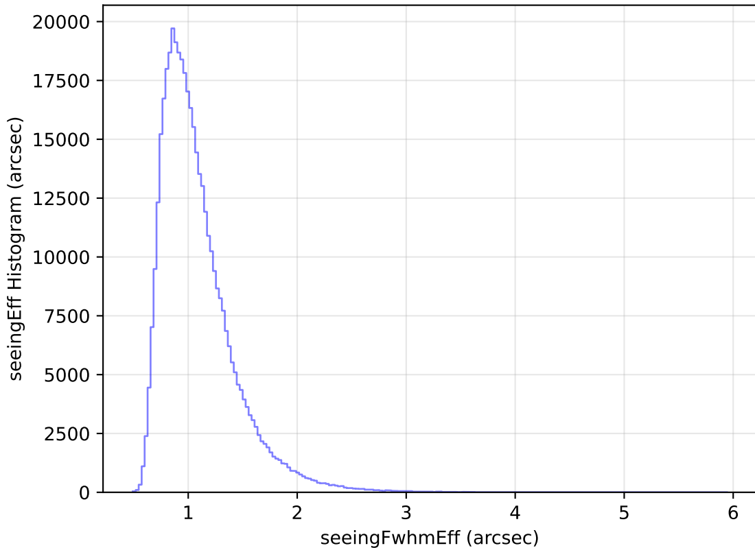
too_elab_heavy_r32_d2_gz_v3.4_10yrs WFD z band: seeingEff Histogram
