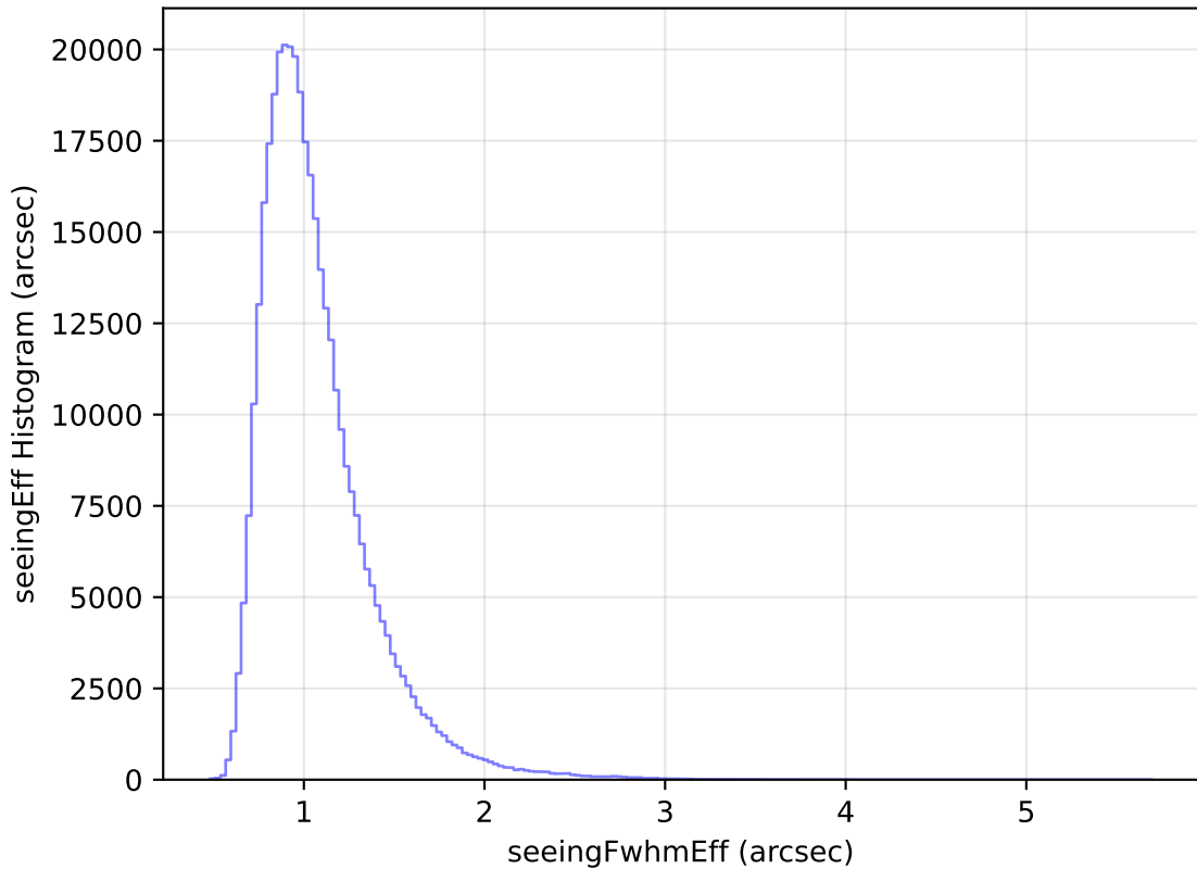
too_elab_heavy_r32_d2_gz_v3.4_10yrs WFD y band: seeingEff Histogram
