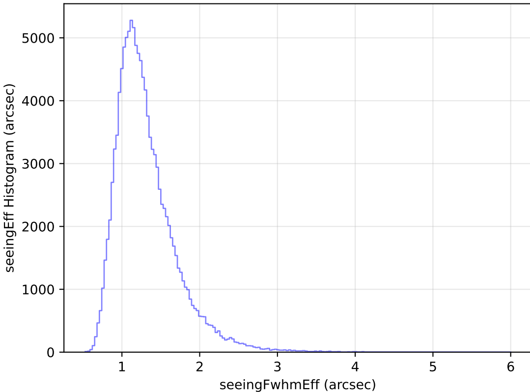
too_elab_heavy_r32_d2_gz_v3.4_10yrs WFD u band: seeingEff Histogram
