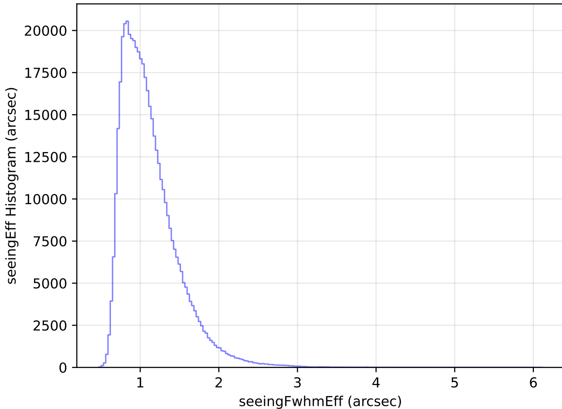
too_elab_heavy_r32_d2_gz_v3.4_10yrs WFD r band: seeingEff Histogram
