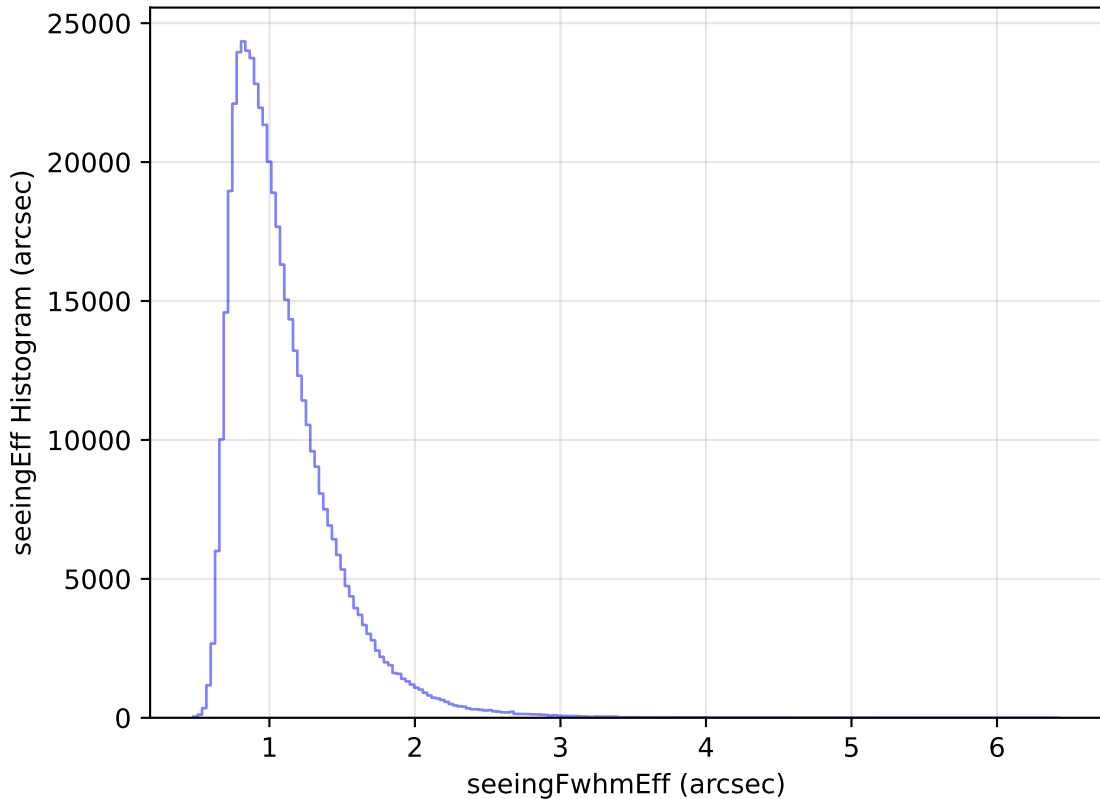
too_elab_heavy_r32_d2_gz_v3.4_10yrs WFD i band: seeingEff Histogram
