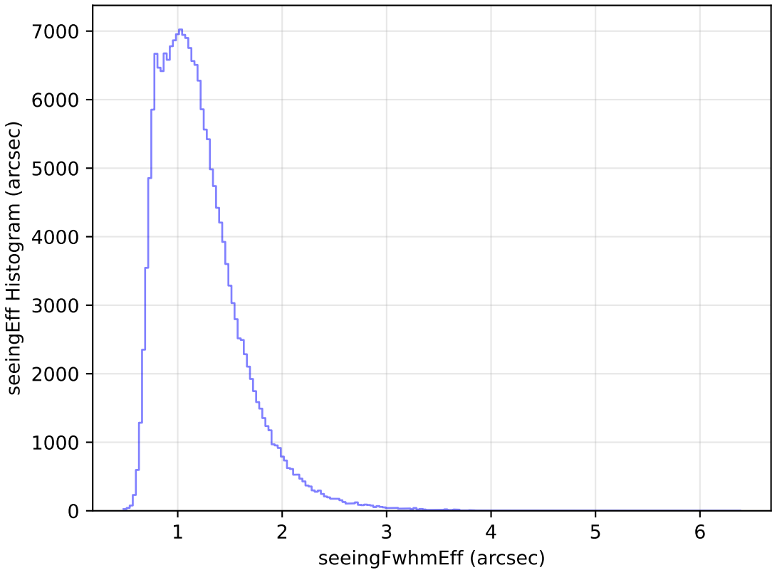
too_elab_heavy_r32_d2_gz_v3.4_10yrs WFD g band: seeingEff Histogram
