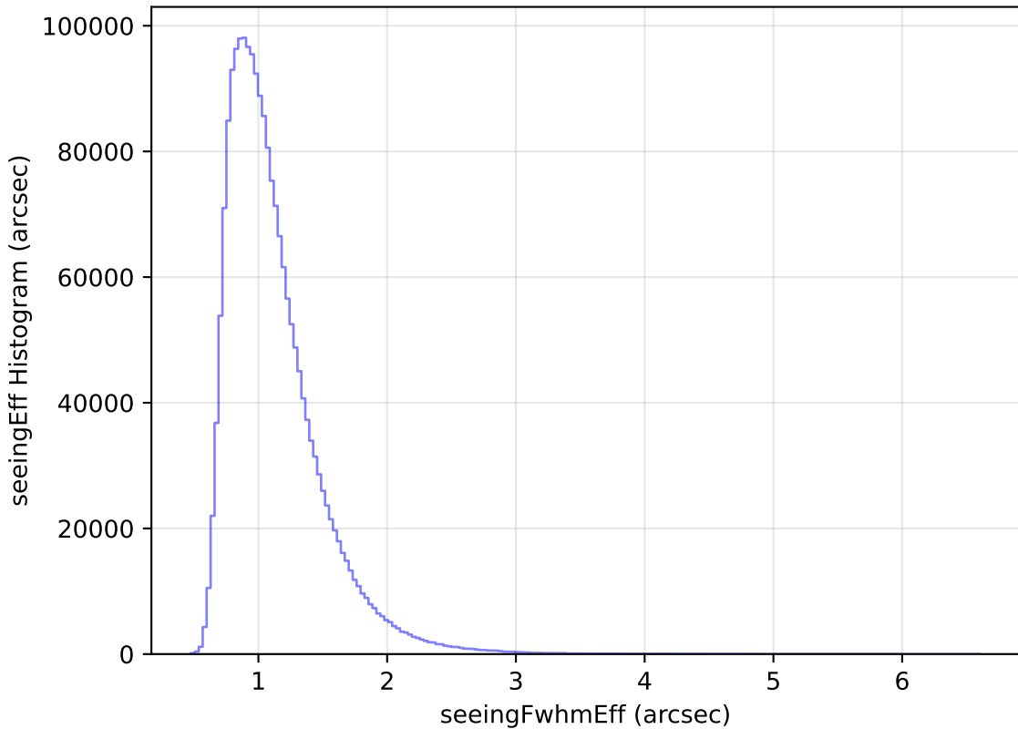
too_elab_heavy_r32_d2_gz_v3.4_10yrs WFD all bands: seeingEff Histogram
