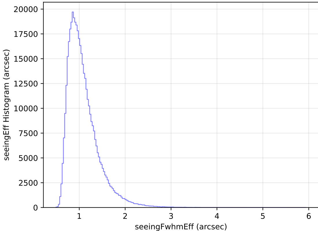
too_elab_heavy_r32_d2_gz_v3.4_10yrs All sky z band: seeingEff Histogram
