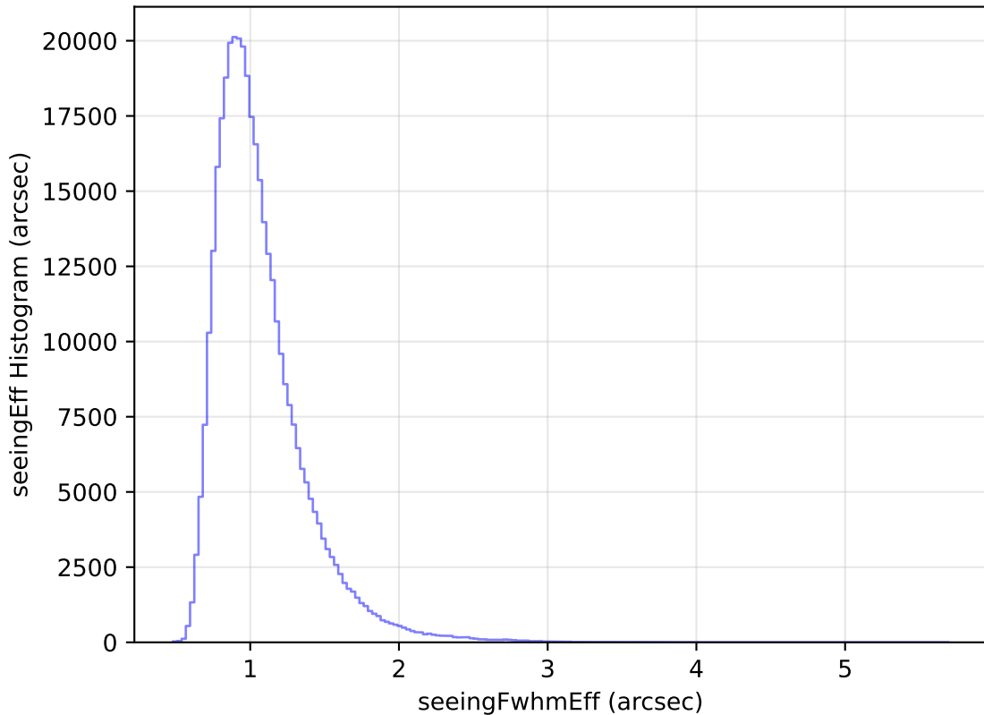
too_elab_heavy_r32_d2_gz_v3.4_10yrs All sky y band: seeingEff Histogram
