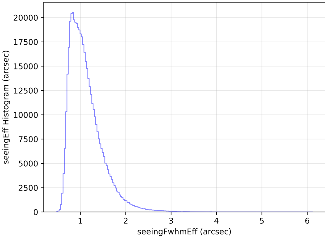
too_elab_heavy_r32_d2_gz_v3.4_10yrs All sky r band: seeingEff Histogram
