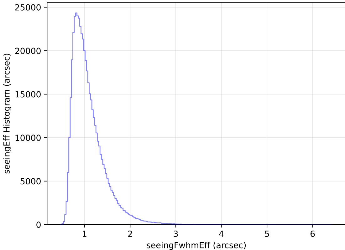
too_elab_heavy_r32_d2_gz_v3.4_10yrs All sky i band: seeingEff Histogram
