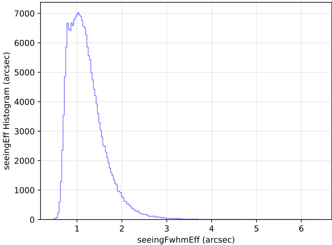
too_elab_heavy_r32_d2_gz_v3.4_10yrs All sky g band: seeingEff Histogram
