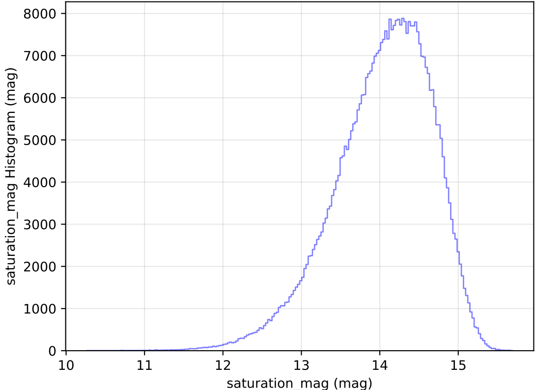
too_elab_heavy_r32_d2_gz_v3.4_10yrs WFD z band: saturation_mag Histogram
