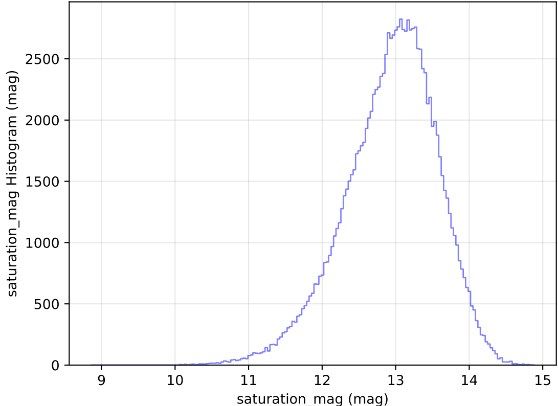
too_elab_heavy_r32_d2_gz_v3.4_10yrs WFD u band: saturation_mag Histogram
