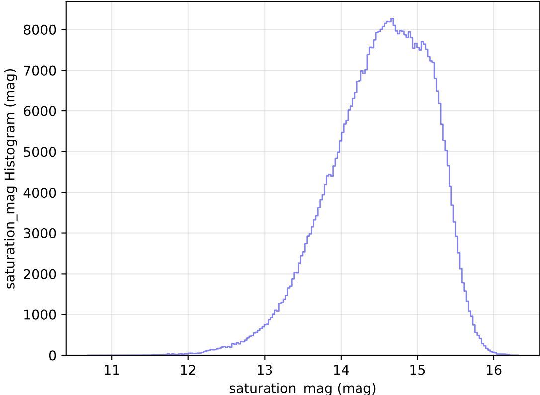
too_elab_heavy_r32_d2_gz_v3.4_10yrs WFD r band: saturation_mag Histogram
