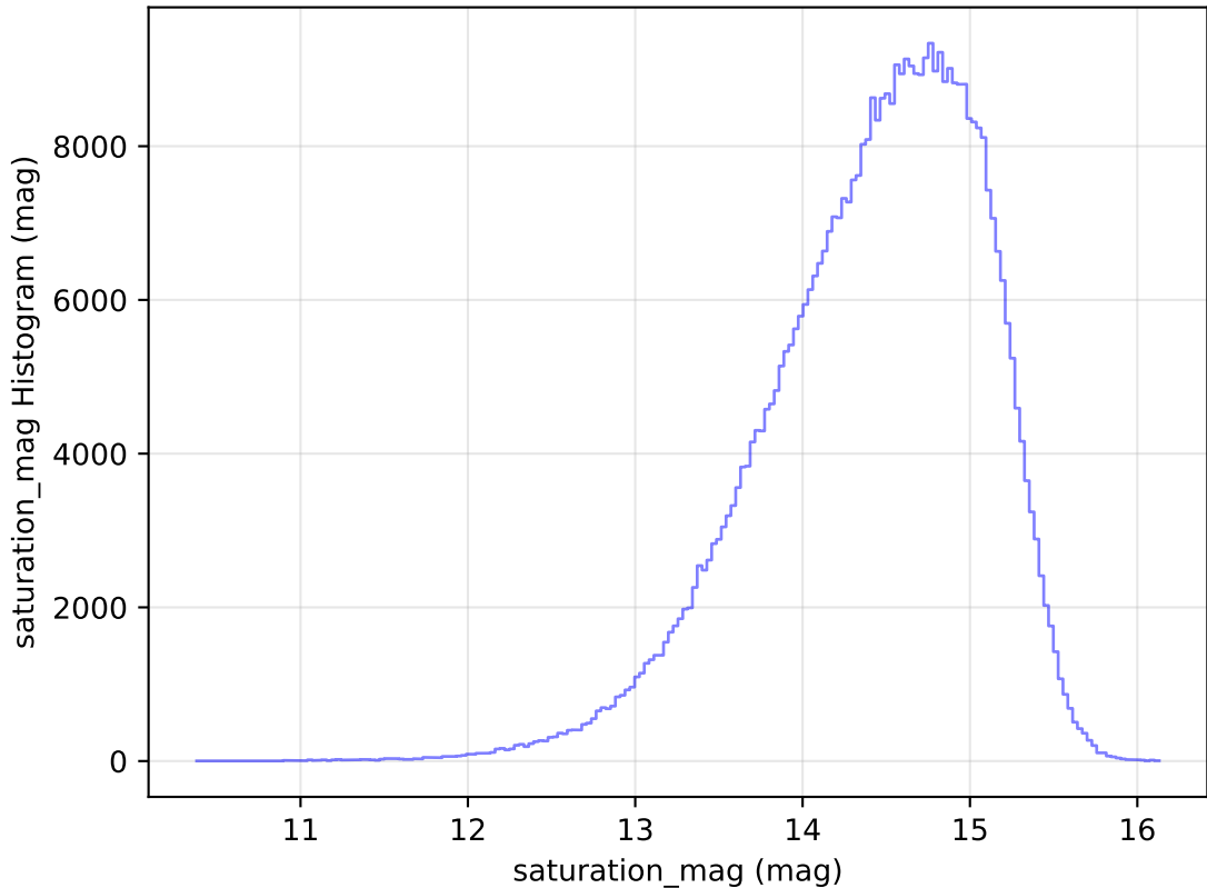
too_elab_heavy_r32_d2_gz_v3.4_10yrs WFD i band: saturation_mag Histogram
