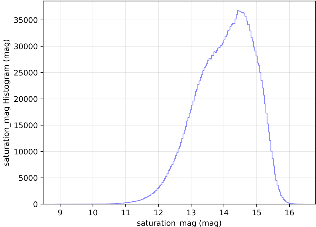
too_elab_heavy_r32_d2_gz_v3.4_10yrs WFD all bands: saturation_mag Histogram
